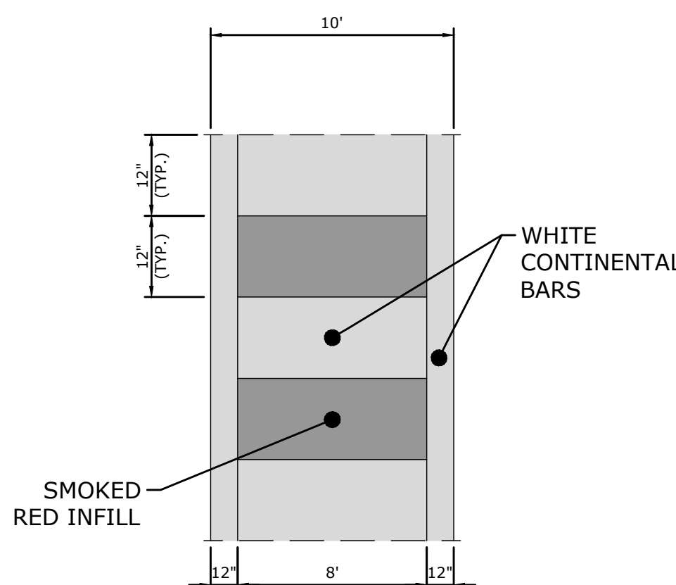
INLAND THERMOPLASTIC CROSSWALK DETAIL NOT TO SCALE
