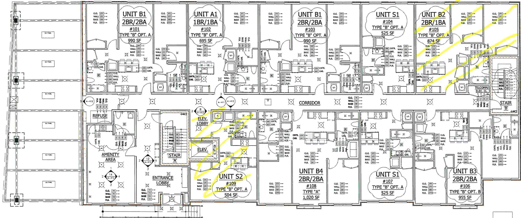
1 REFLECTED CLG. PLAN - FIRST FL. SCALE: 1/8" = 1'-0"
