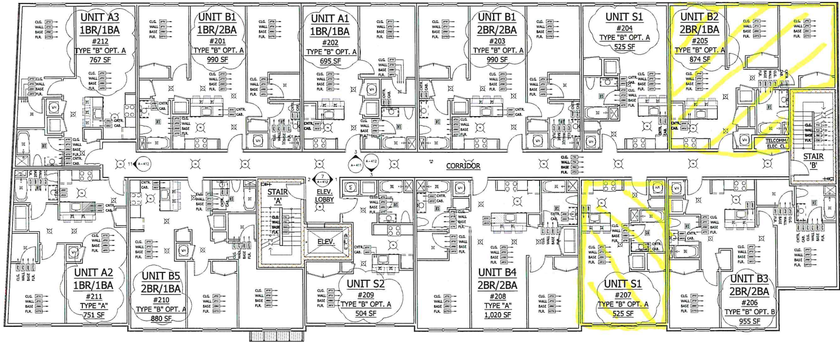
1 REFLECTED CLG. PLAN - SECOND FL. SCALE: 1/8" = 1'-0"
